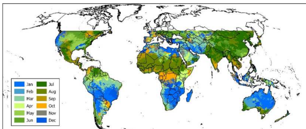
Fig. 2. Peak month of precipitation, based on highest mean, 1981–2020.
