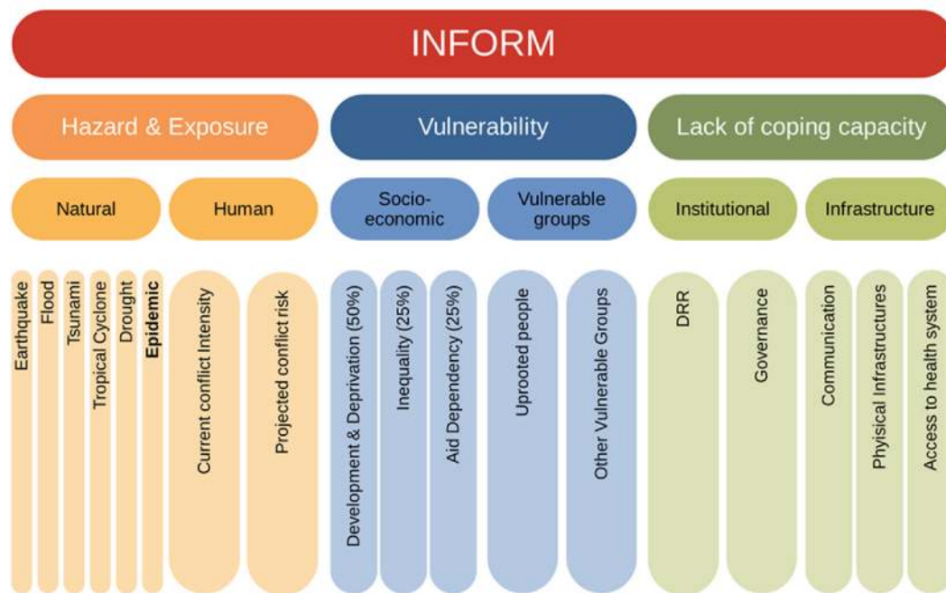
Fig. 1. Components of INFORM risk index (source: INFORM, 2020 ).
