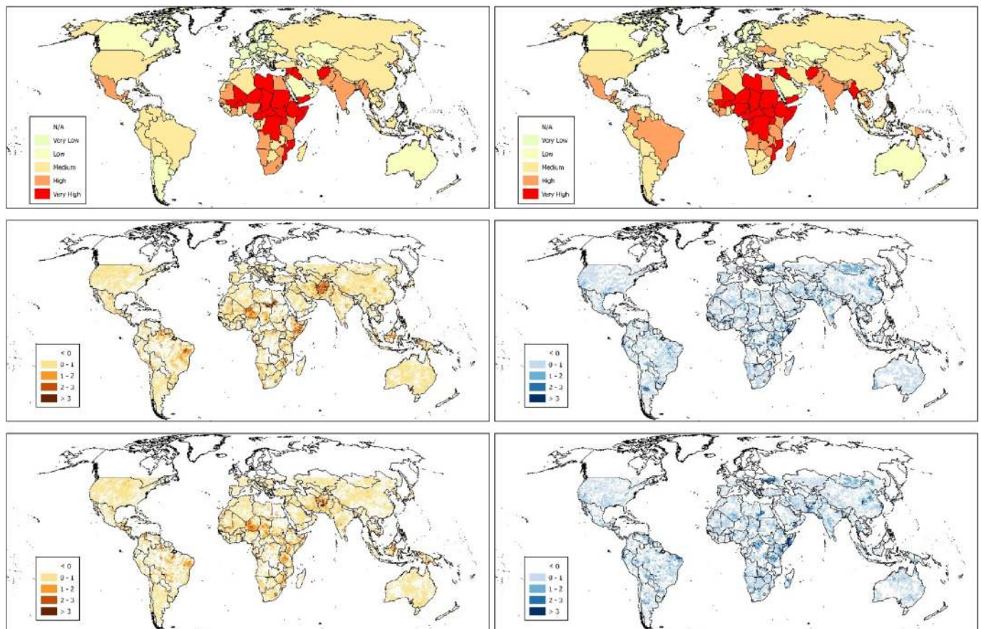
Fig. 4. Country-level risk score (INFORM, 2020; top), suitability score for peak month (middle) and peak season (bottom), for droughts (left) and floods (right).
