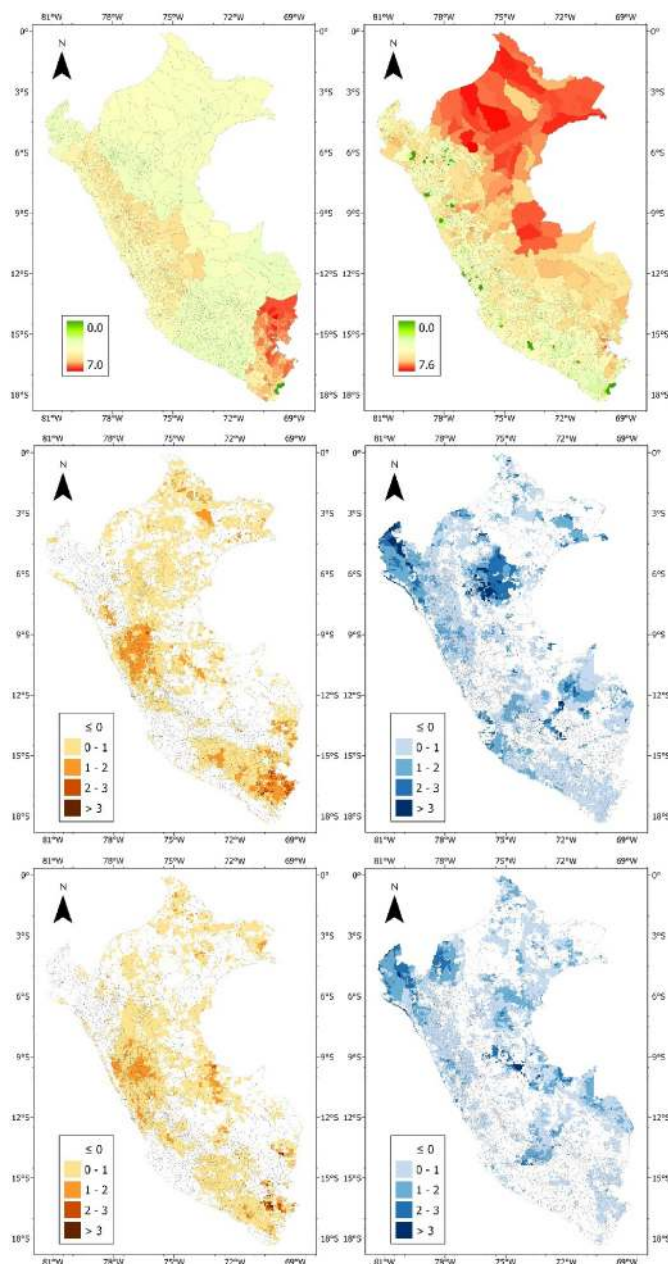
Fig. 6. Peru: risk score (top), suitability score for peak month (middle) and peak season (bottom), for droughts (left) and floods (right).
