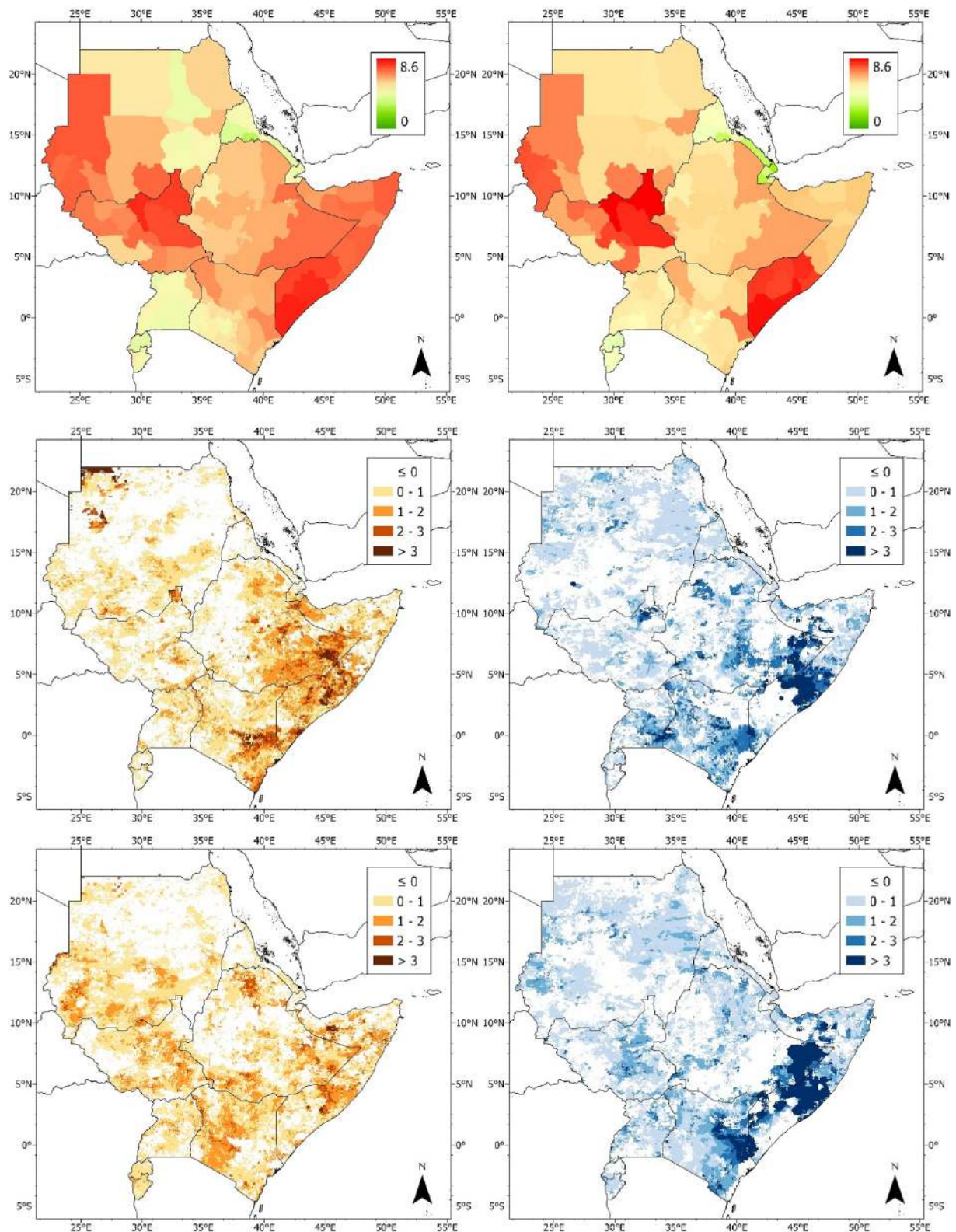
Fig. 5. Greater Horn of Africa: risk score (INFORM, 2020; top), suitability score for peak month (middle) and peak season (bottom), for droughts (left) and floods (right).
