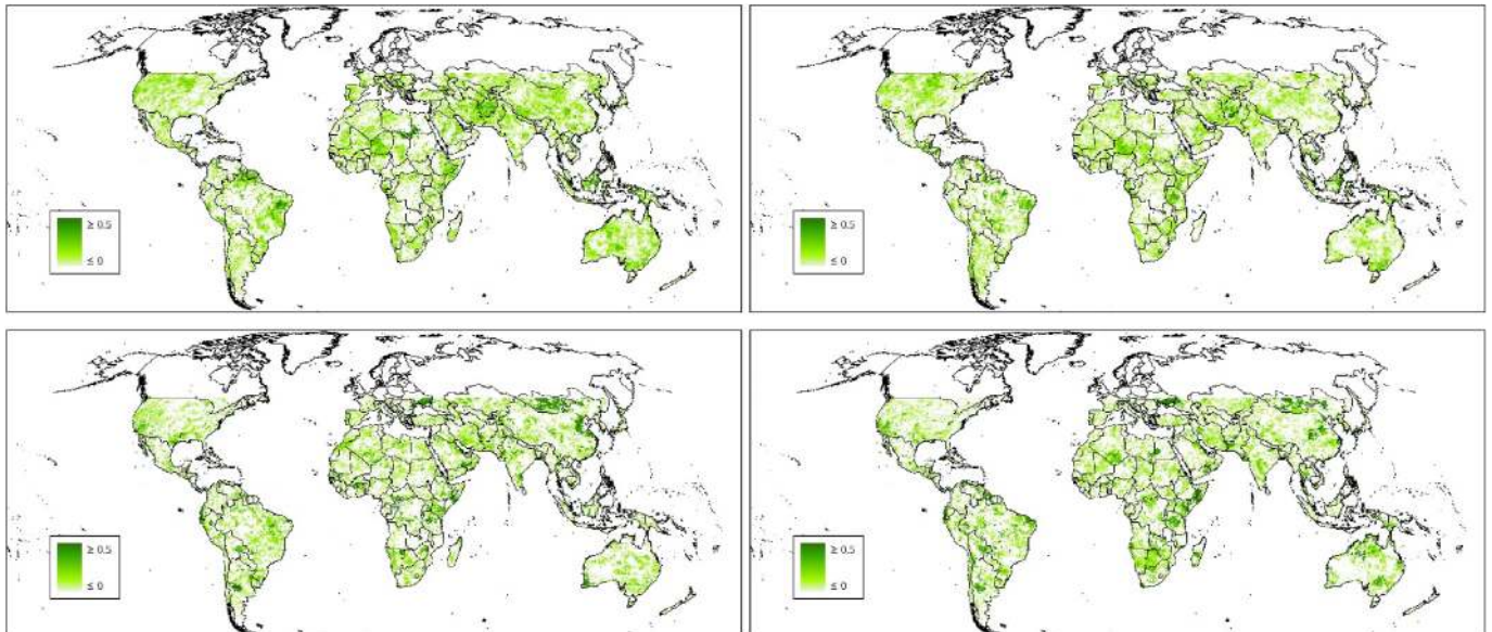
Fig. 3. Maximum Brier skill scores for NCEP and ECMWF forecasts ( BSS_{max} ), for peak month (left) and season (right), and for the 15th percentile (top; droughts) and 95th percentile (bottom; floods) of precipitation.
