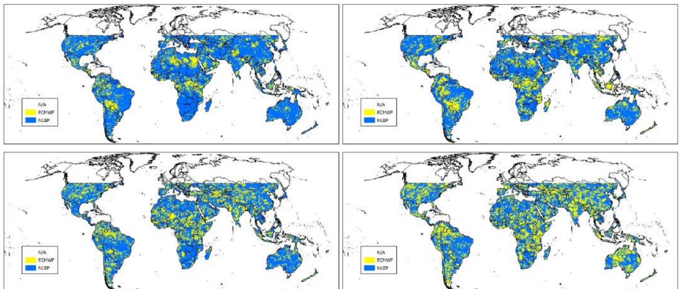
Fig. A1. Forecast source with higher Brier skill score for peak month (left) and season (right), and for the 15th percentile (top; droughts) and 95th percentile (bottom; floods) of precipitation
